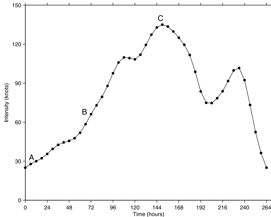
Figure 1. Example of intensification for a typical TC. Intensification rates I_1 and I_2 are determined between the points A-B and B-C respectively.
