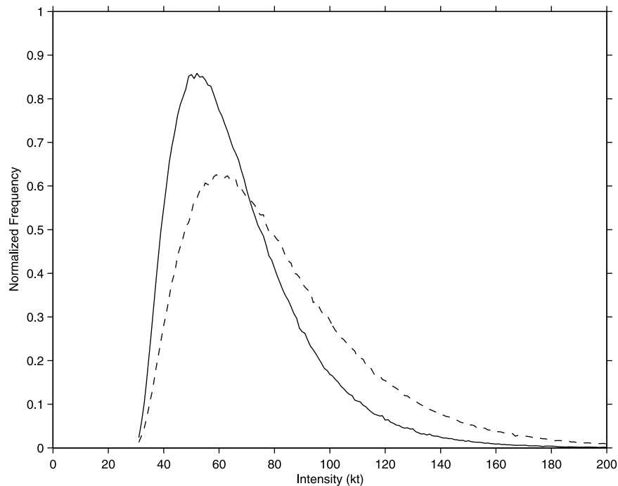
Figure 3. Simulated intensity distribution of global cyclones (solid line), and the same with 30% increase in average intensification rate (dashed line).
