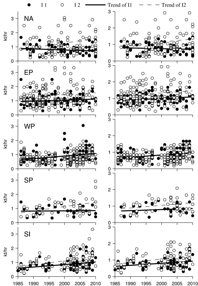
Figure 2. Variation of intensification rates I_1 (dark circles) and I_2 (open circles) with time. (left) All valid observations for five basins, (right) same as left panel but with top 5% values of I_1 and I_2 removed from the data.
